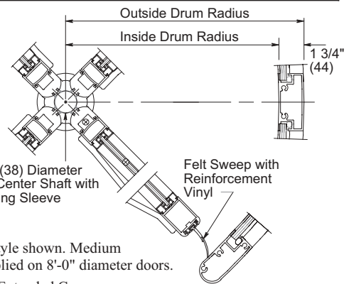
Horizontal Section
