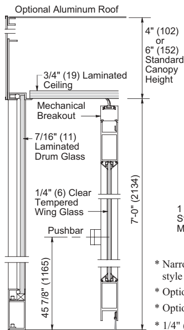
Vertical Section
