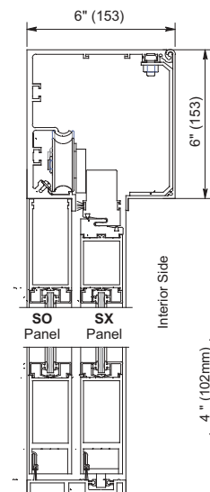
Vertical Section
