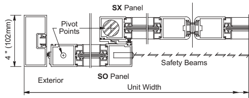
Horizontal Section
