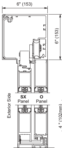
Vertical Section
