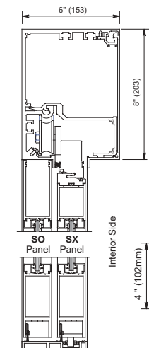
Vertical Section
