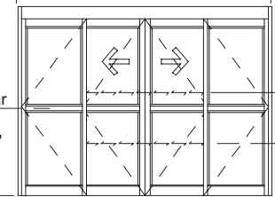
Type SO-SX-SX-SO
