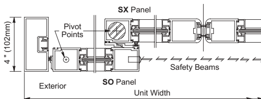
Horizontal Section
