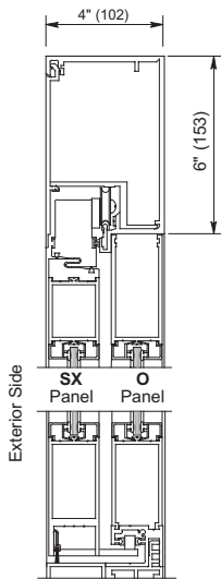
Vertical Section
